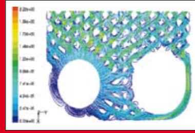
Simulation is one of the most important stages in the development of new and existing CBHEs. The ability to evaluate different plate patterns by simulating flow rate and directions offers great opportunities for improved functionality.
